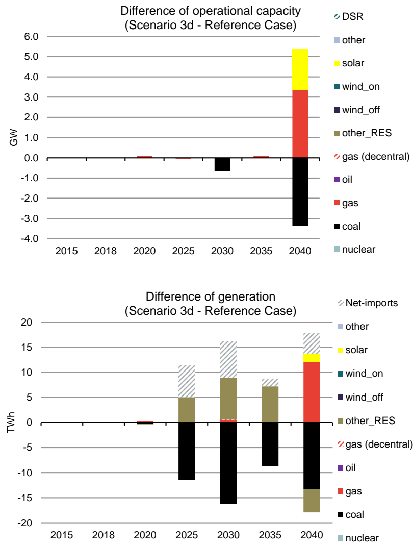
Figure 59. Impact on the Dutch electricity supply (Scenario 3d)
