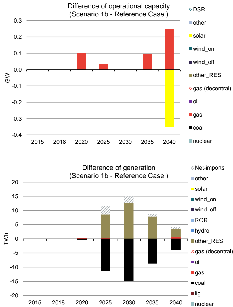
Figure 44. Impact on the Dutch electricity supply (Scenario 1b)
