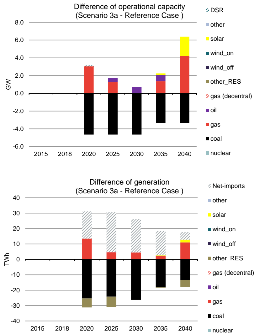
Figure 50. Impact on the Dutch electricity supply (Scenario 3a)
