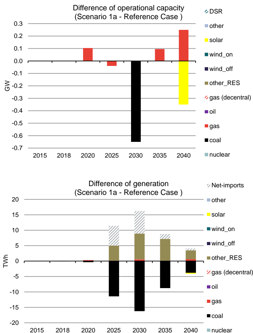
Figure 41. Impact on the Dutch electricity supply (Scenario 1a)
