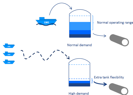
Figure 16. LNG tank flexibility.
