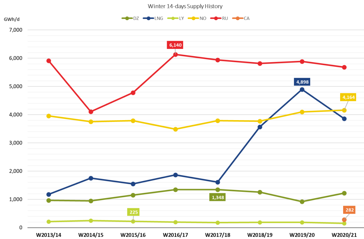
Figure 11. 2-week supply history.
