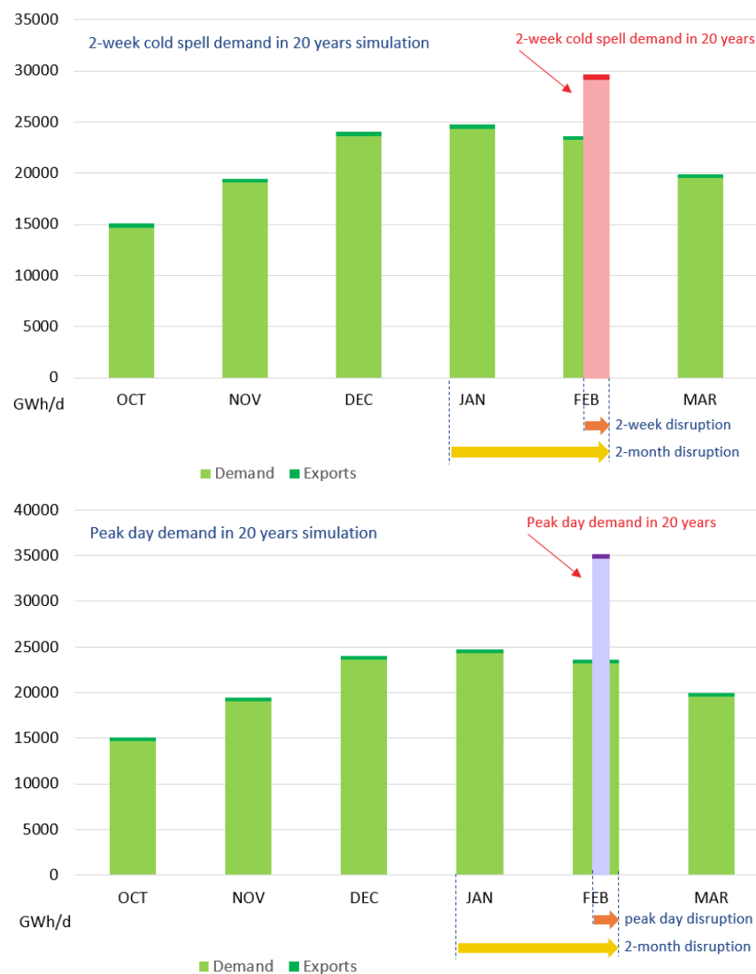
Figure 7. Demand assumption and disruption timeframes.
