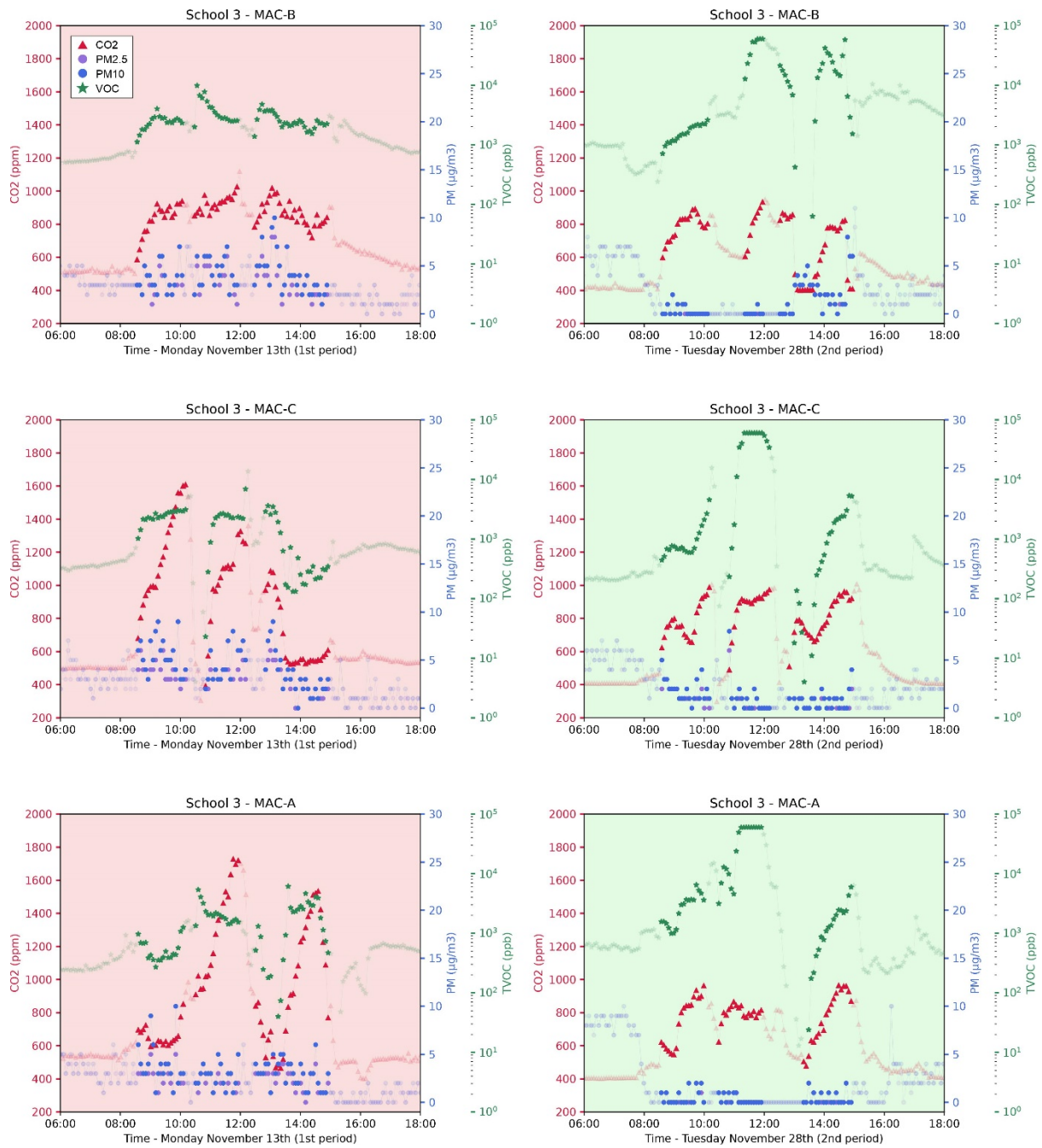
Figure Appendix B3. Time evolution of PM2.5, PM10, CO2, and VOC concentrations in the classrooms monitored in School3, between 06:00 and 18:00 on 1) a day during the 1st period: Monday November 13th, 2023 (left) and 2) a day during the 2nd period: Tuesday November 28th, 2023 (right). The background colour indicates whether the MAC is turned on (green) or off (red) on that day. Light data points correspond to unoccupied hours.
