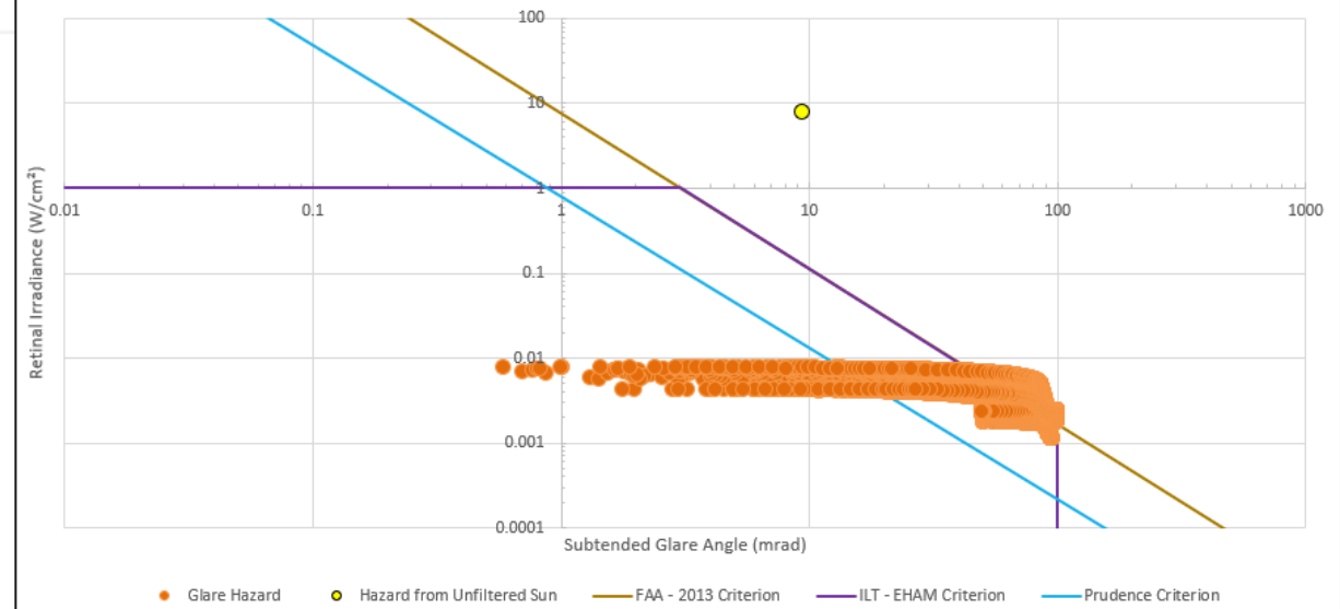
Glare Hazard Plot RWY 18R: FP 0-8 miles (Field A, 222° orientation)
