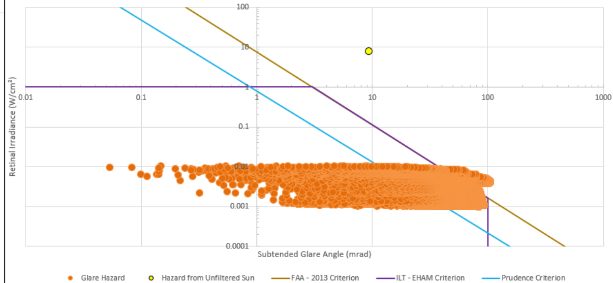
Glare Hazard Plot RWY 18R: FP 0-8 miles (Field A, 42° orientation)
