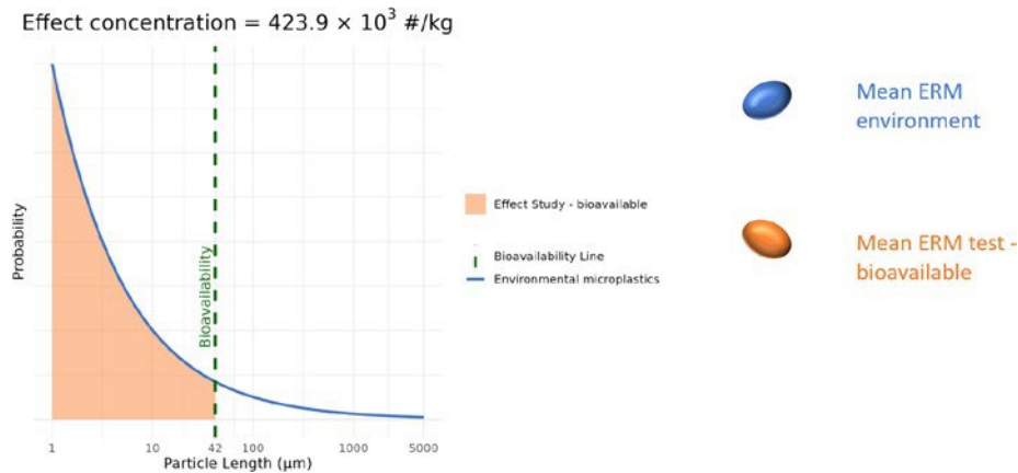
Figure A2.4 Illustration of power law size distribution representing environmental microplastics in size range 1 to 5000 \mu\text{m} (blue line) and the size range used in an effect study (orange shading).
