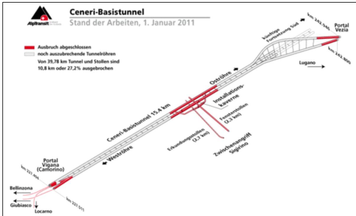
Figure 30: Drilling works at Ceneri Tunnel (01.01.2011)
