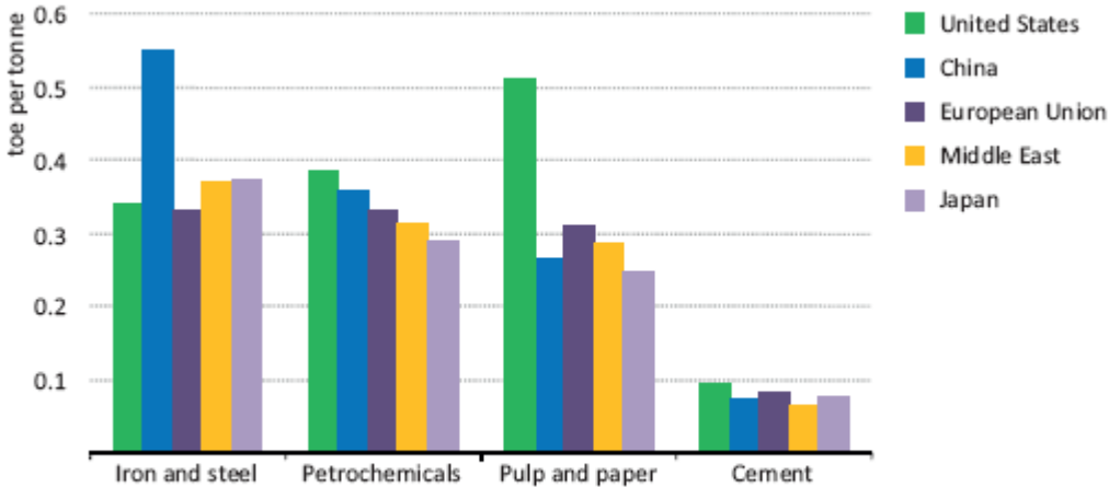
Figure 27. Energy intensity by sub-sector and region, 2011
