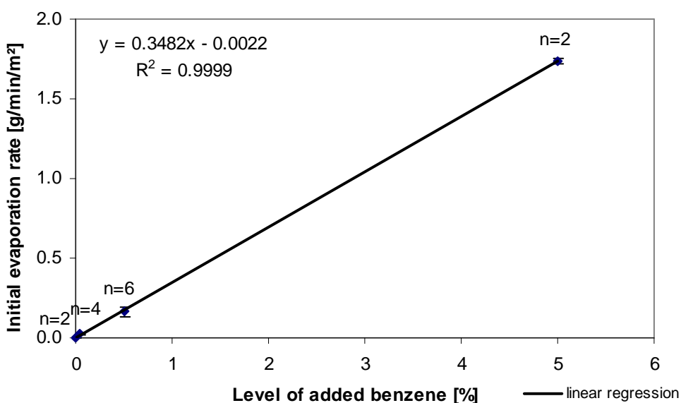
Figure 4-1: Estimated passive initial benzene emission rate by benzene content level in PX-10.
