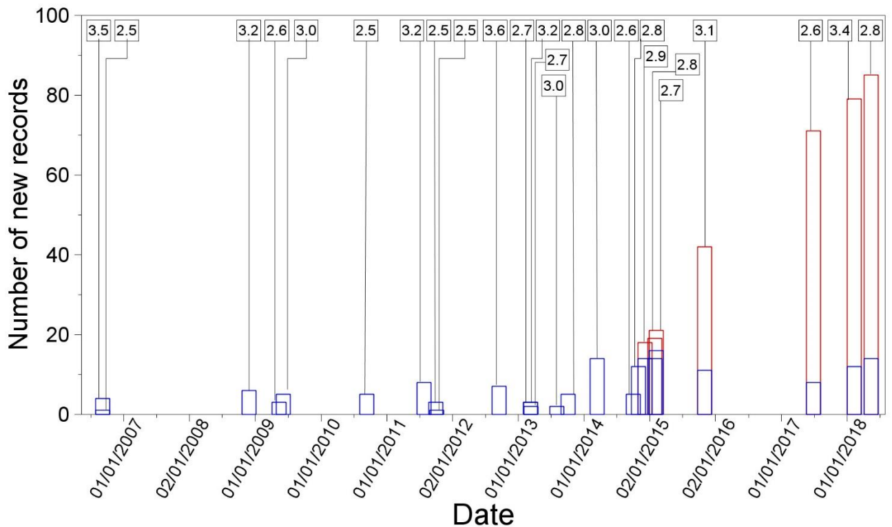
Figure 2.2. Diagram illustrating the timing of earthquakes of M_L \geq 2.5 in the Groningen field until the end of 2018 and the number of records yielded by the permanent KNMI network (B-stations, blue) and by the expanded borehole geophone network (G-stations, red).
