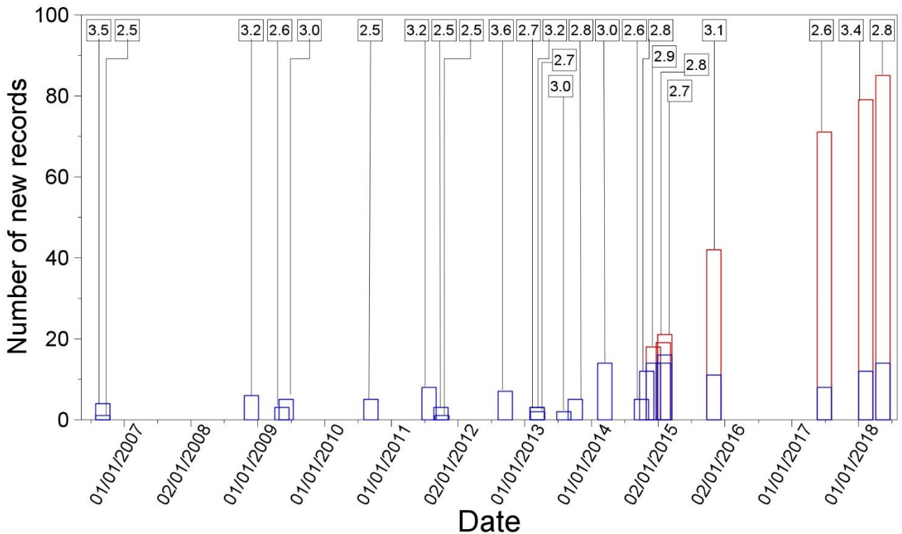
Figure 4.2. Diagram illustrating the timing of earthquakes of M_L \geq 2.5 in the Groningen field until the end of 2018 and the number of records yielded by the permanent KNMI network (B-stations, blue) and by the expanded borehole geophone network (G-stations, red).
