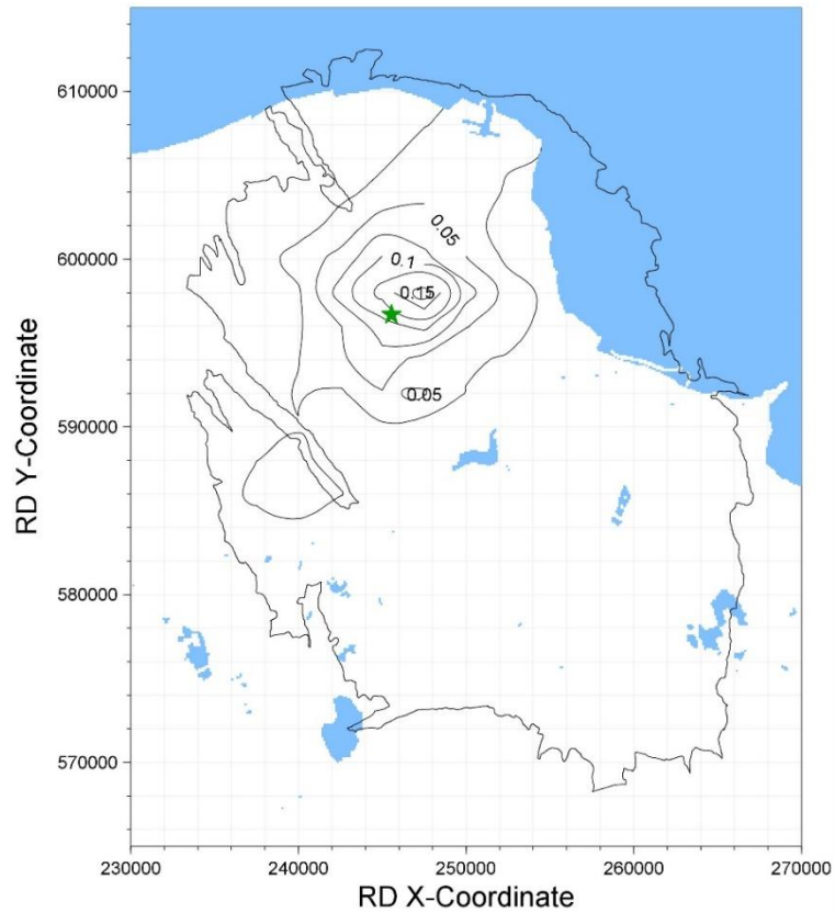
Figure 5.9 Contours of MaxRot PGV recorded during the M_{1.5} (upper) and M_{1.2} (lower) Zeerijp events. Units are cm/s; unnumbered lines represent increments of 0.025 cm/s
