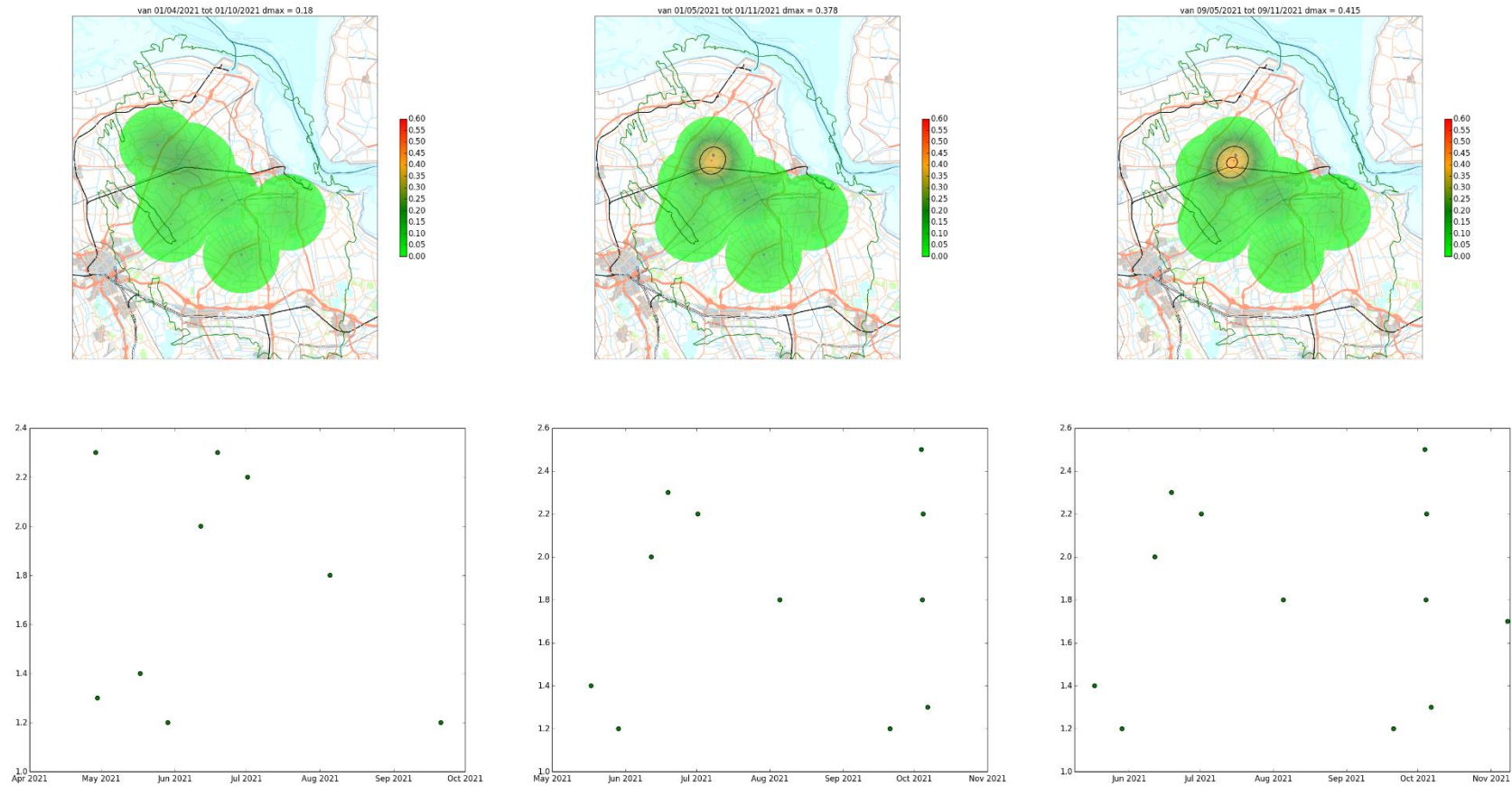
Figure 6.3 This panel shows the earthquake density (above) en the magnitude of the earthquakes versus time (below) for three different time periods. Left this is shown for the 6 months preceding 1 st October 2021, in the centre for the 6 months preceding 1 st November 2021 and to the right the period preceding 9 th November 2021.
