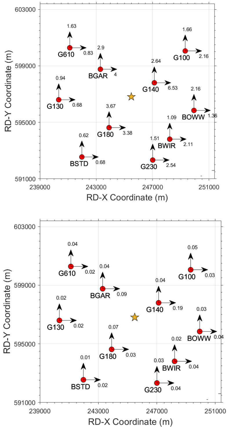
Figure 4.7. Horizontal components of PGA (upper) and PGV (lower) recorded during the Zeerijp earthquake at epicentral distances of less than 6 km; units are cm/s 2 and cm/s, respectively.
