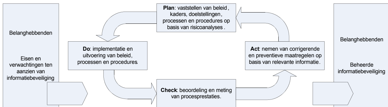
Plan-Do-Check-Act model
