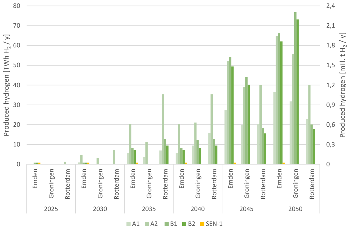
Figure 24: Hydrogen production quantities in metric tons per year for the different scenarios and reference years at Emden, Groningen and Rotterdam
