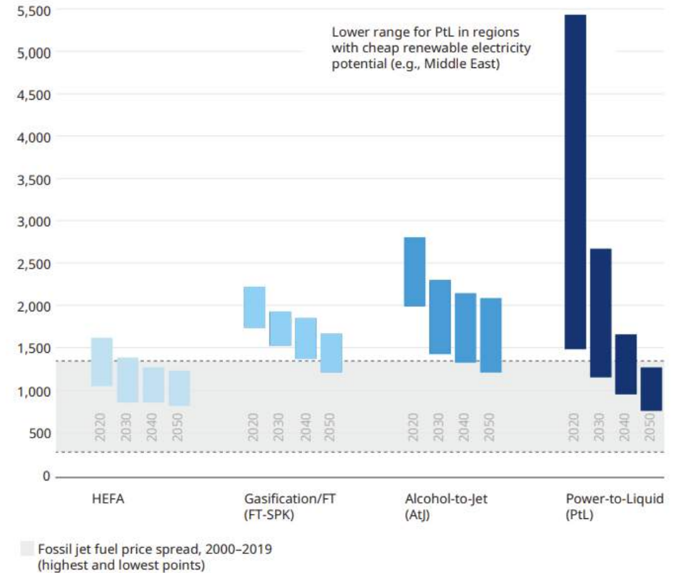
Exhibit 9: Cost profile of SAF pathways between 2020 and 2050
