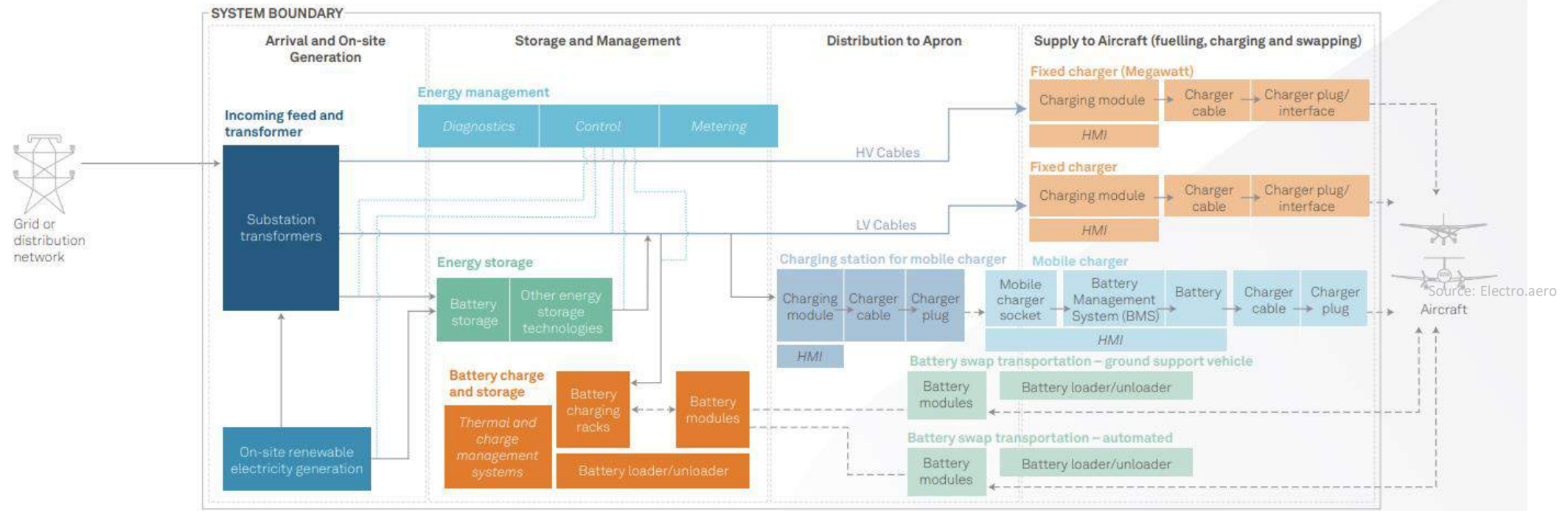
Figure 6: Electric system architecture
