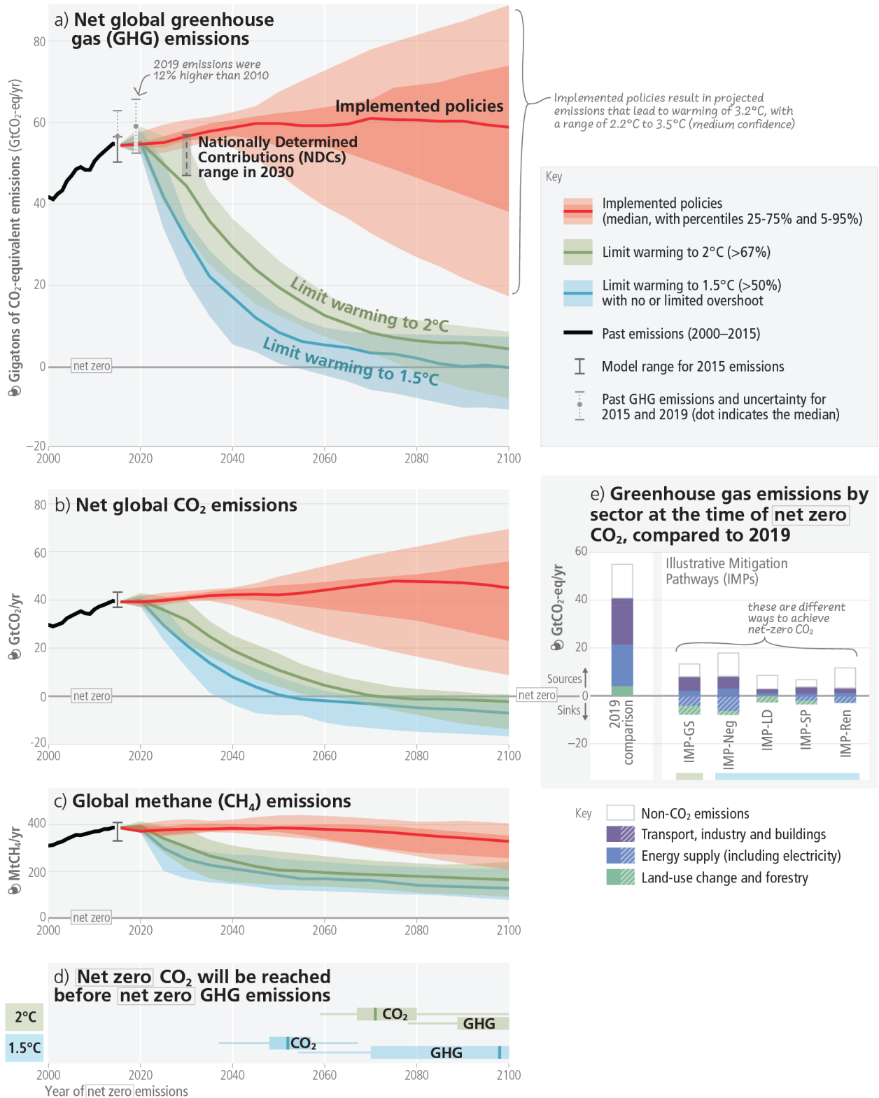
Figure SPM.5: Global emissions pathways consistent with implemented policies and mitigation strategies. Panel (a), (b) and (c) show the development of global GHG, CO 2 and methane emissions in modelled pathways, while panel (d) shows the associated timing of when GHG and CO 2 emissions reach net zero. Coloured ranges denote the 5th to 95th percentile across the global modelled pathways falling within a given category as described in Box SPM.1. The red ranges depict emissions pathways assuming policies that were implemented by the end of 2020. Ranges of modelled pathways that limit warming to 1.5°C (>50%) with no or limited overshoot are shown in light blue (category C1) and pathways that
