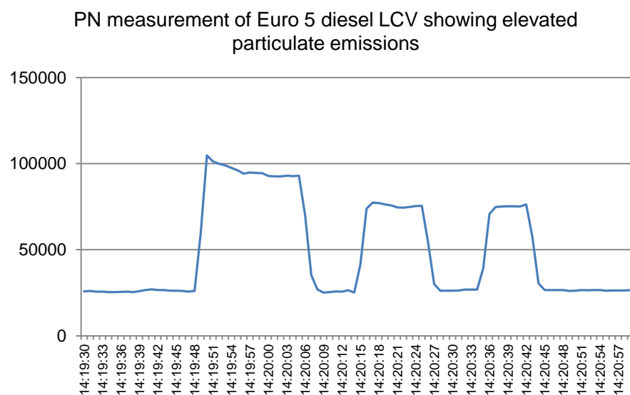
Figure 14 PN measurement on a Euro 5 LCV showing elevated particulate emissions. The measurement was performed three times to check for reproducibility.
