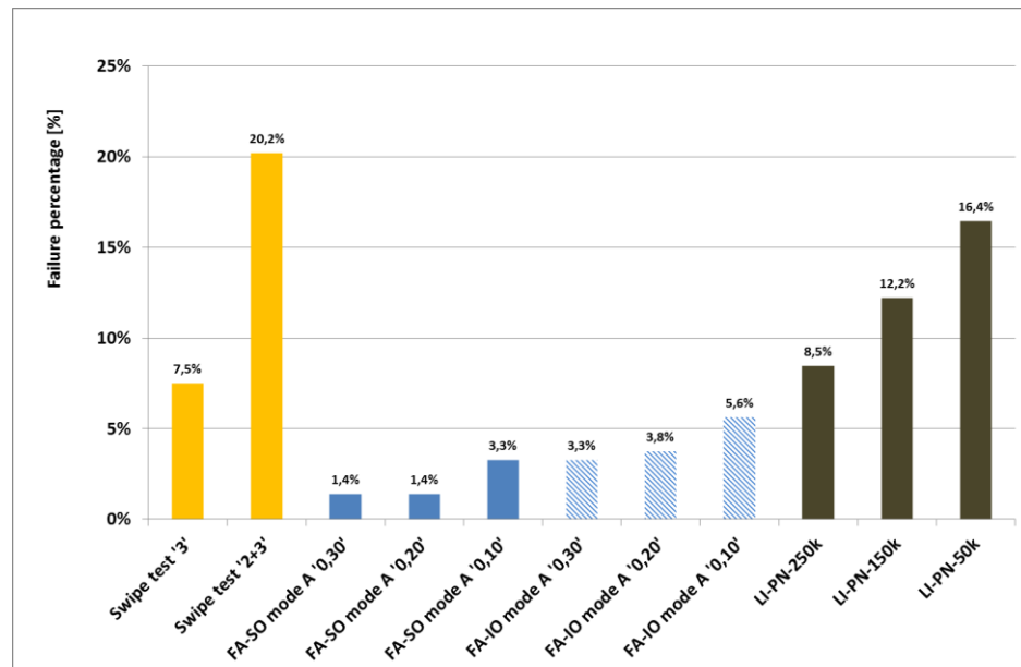
Figure 44: Percentages of DPF failures based on different test procedures and limit values
